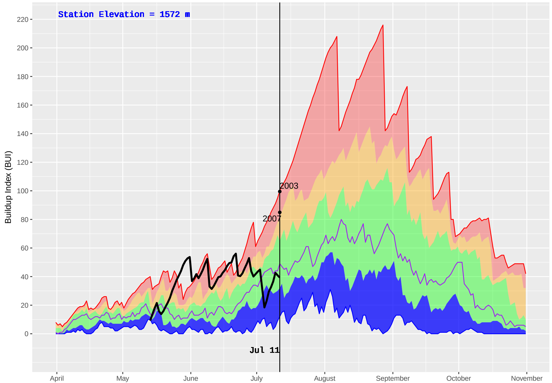
NEGRO CREEK (789) : Historical (2001–2016) and Current (2018) Noon Buildup Index (BUI)
